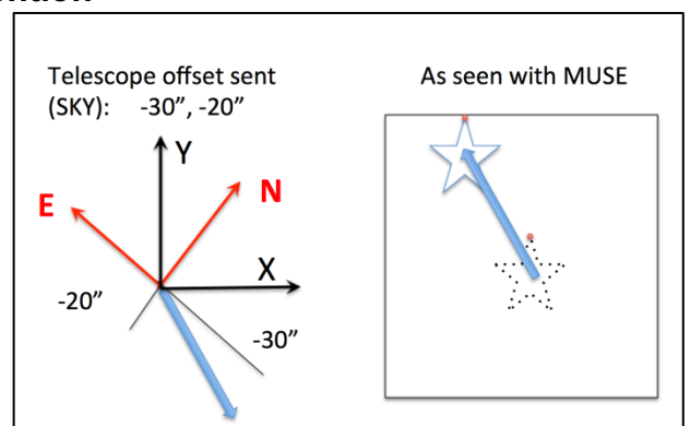
Figure 23: Offset conventions for MUSE. We summarize here the main definitions
