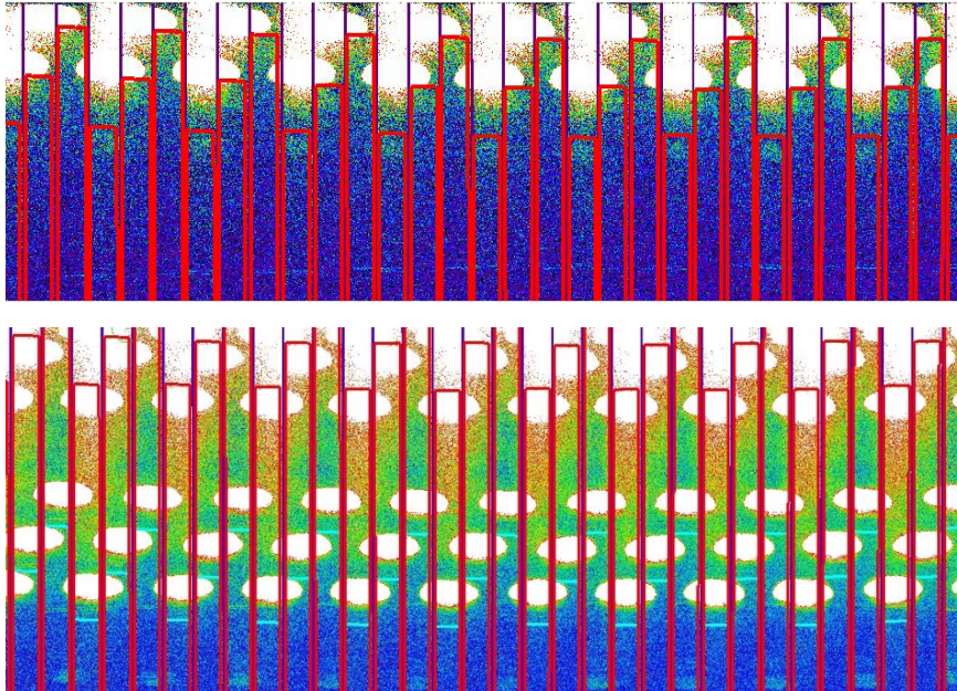
Figure 18: Second order effect in nominal (top panel) and extended (bottom panel) modes, shown here for a bright exposure with arc lines. The red boxes mark the slice limits up to 930 nm. The impact of second order is visible as the white ellipses illuminating the top of the detector. The nominal instrument mode is not affected by contamination, but it is more significant in the extended instrument mode.
