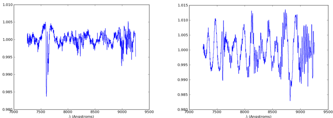
Figure 19: Fringing measured in the red, measured on normalised flat-field frames. (left) WFM, (right) NFM.
