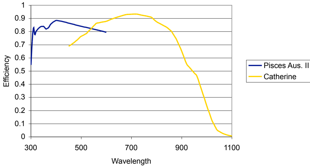
Figure 8: UVB/VIS detector efficiency.
