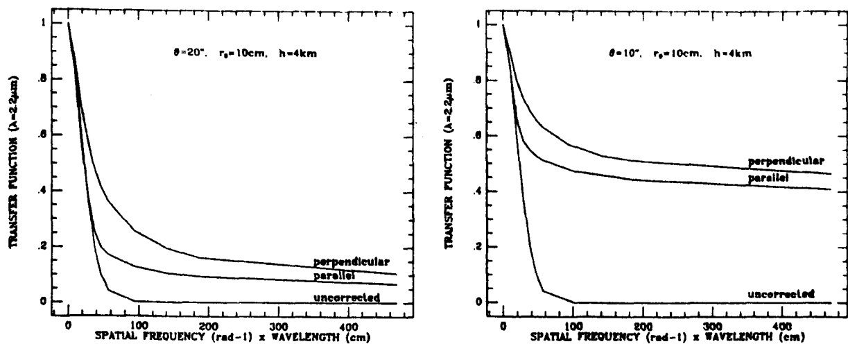
Figure A1-2 : Corrected MTF at λ = 2.2 μm, using a reference star at θ = 10 and 20" (seeing 1", turbulent layer at h = 4 km). The size of the isoplanatic field is linear with h -1 (Roddier and Roddier, 1986). Abcissae as in Fig.A1.1. Note the slight anisotropy of the correction.
