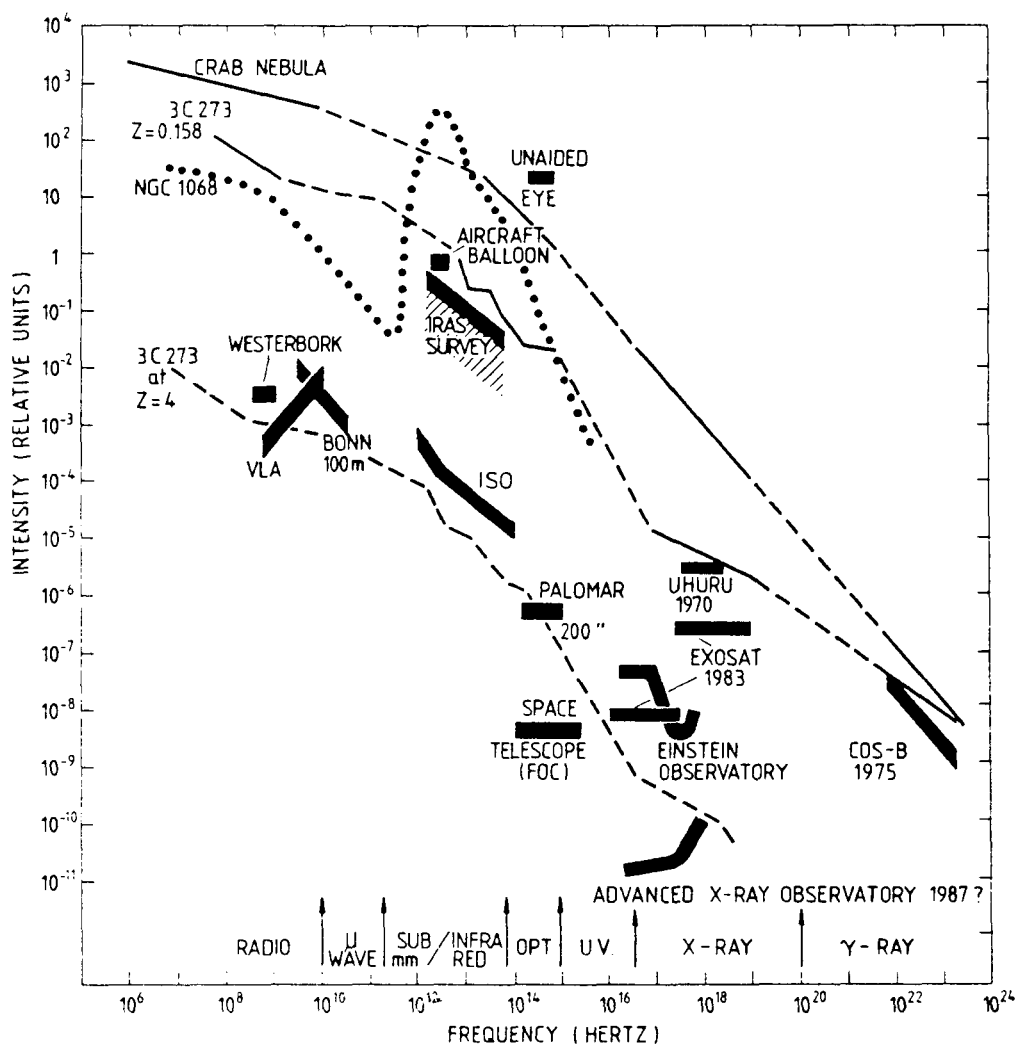
Figure 1.1-1 : Overview of the relative sensitivity of existing or planned instruments at different wavelengths. The spectrum of a quasar (3C 273) and of an active galactic nucleus (NGC 1068) with thermal and non-thermal components are given for reference.
