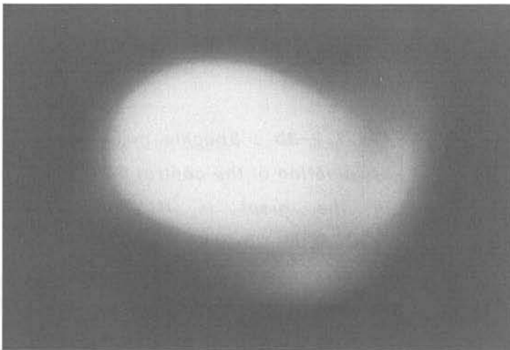
Fig. 1.2-2 : Image of \alpha Ori at 535 nm ( \Delta\lambda \sim 1 nm). The image was reconstructed from interferometric observations made at the 3.6 m CFH Telescope in Hawaii, using the Gull and Daniel algorithm. Circumstellar shell is obvious (Roddier and Roddier 1985).
