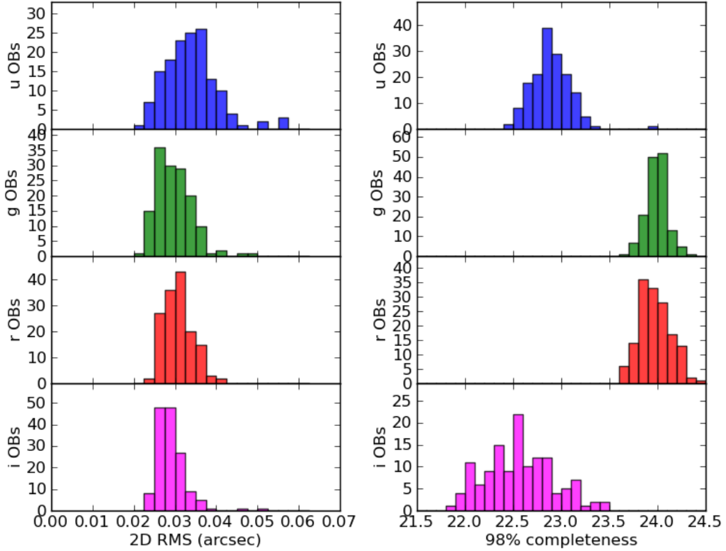
Figure 8: Overview of the astrometric quality and completeness of KiDS-ESO-DR1 and KiDS-ESO-DR2 (all data contained in the multi-band catalogue). Left: median relative astrometric offsets between the dithers in a coadd. Right: 98% completeness magnitude distributions for all tiles. In both columns the panels correspond to u, g, r, and i from top to bottom.
