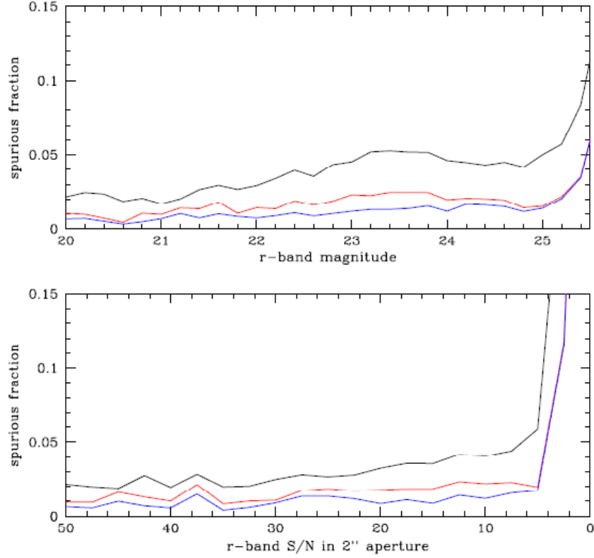
Figure 9: Spurious source contamination in the overlap between KiDS-ESO-DR2 and the CF-HTLS-W2 field (this corresponds to the KiDS tiles KiDS_135.0_-1.5 and KiDS_136.0_-1.5). Top: spurious fraction vs. r -band magnitude ( MAG_ISO ). Bottom: spurious fraction vs. signal-to-noise in a 2'' aperture. The black line corresponds to all sources, while the red line excludes sources in masked areas, and the blue line excludes sources in masked areas and sources with a non-zero SExtractor flag.
