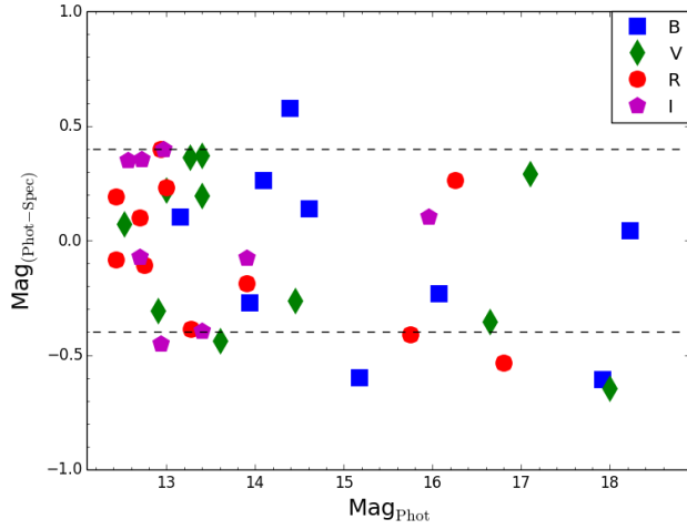
Fig 1: Synthetic magnitudes as measured from flux-calibrated spectra (Gr#11 and Gr#16) compared to the photometric magnitude at the same epoch for SN2013ej (Yuan et al., in prep.). Mag_{Phot} is the calibrated photometric magnitude and the y-axis is the difference between this and the synthetic photometry measured from the flux calibrated spectra. Colours and symbols indicate filters. The mean of all the values is -0.058 with a RMS of 0.360.
