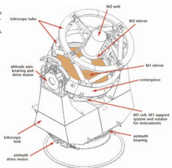
Figure 7: Diagram of telescope structure showing the major components.
