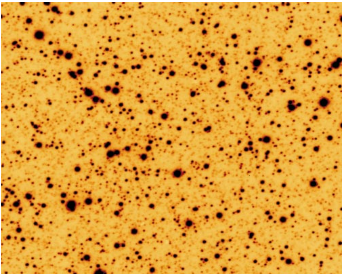
Omega Centauri, obtained with the VLT UT1 on May 16, 1998. (For more details, see text in box on page 3.)
