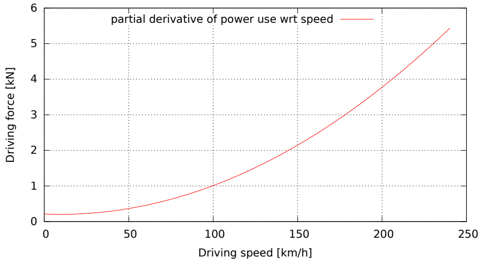
Tesla Model 3 RWD driving force vs driving speed
