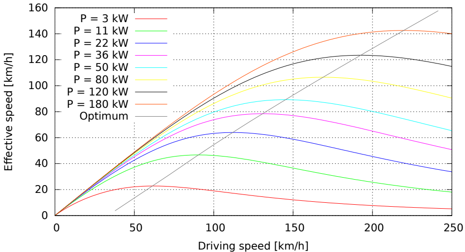
Tesla Model 3 RWD Effective speed vs driving speed at various charging speeds
