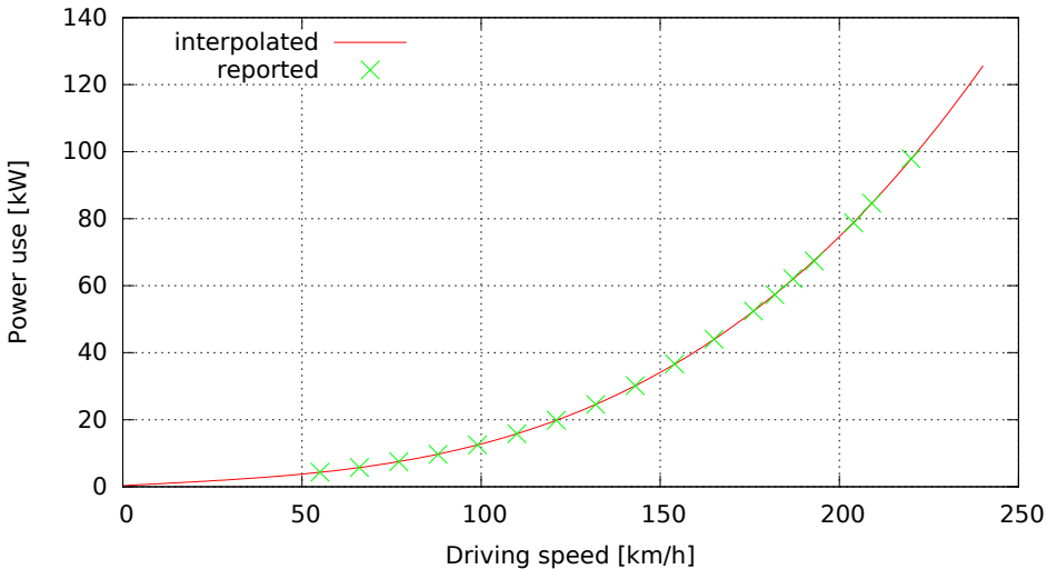
Tesla Model 3 RWD power use vs driving speed
