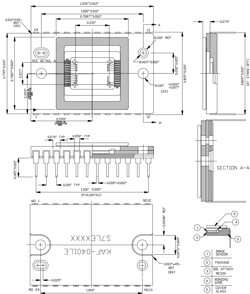
Figure 2 - Package Drawing
